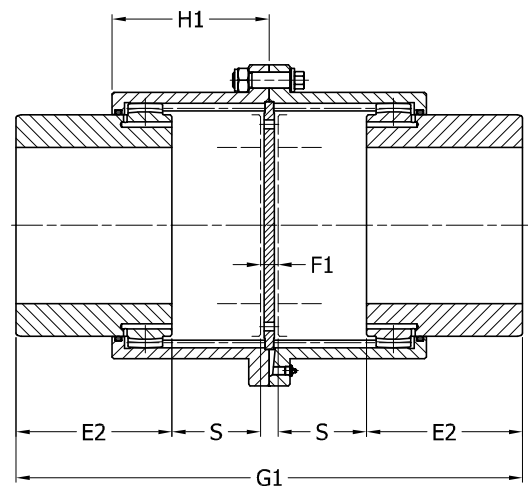
Type SGG - Double Slide = S + S
