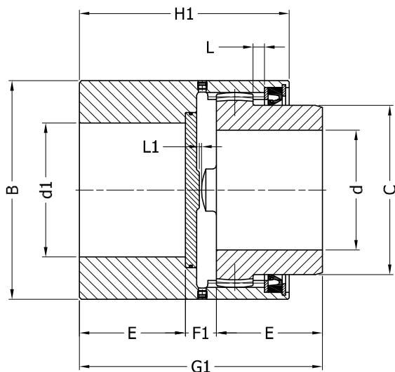
Fig.3 - Example : size 335 Gear Coupling SGC-335.3.R Gear Coupling SGC-335.6.R
