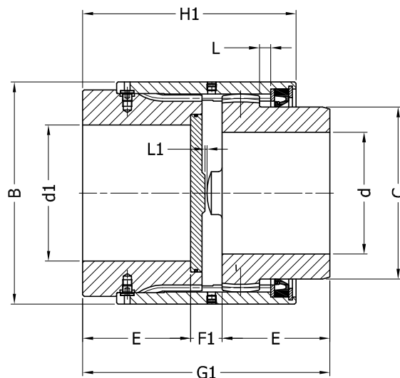
Fig.4 - Example : size 335 Gear Coupling SGC-335.3.S Gear Coupling SGC-335.6.S
