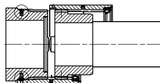
Fig.9 - Fully opened plugs, retain stopped sleeve on the hub.
