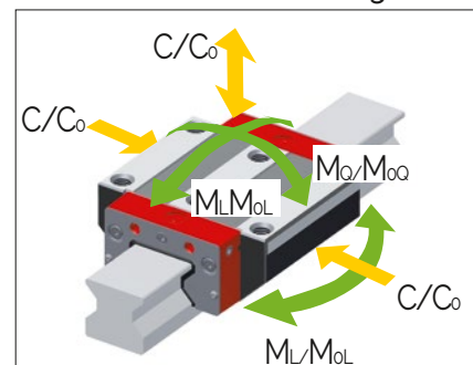
AMSABS 3B W 35 Load rating
