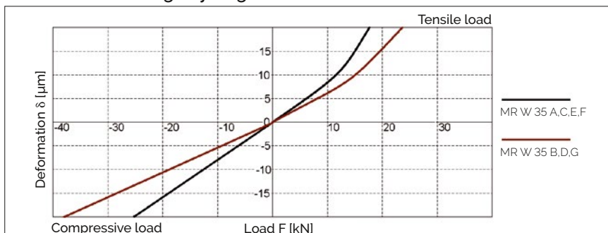
AMSABS 3B W 35 Rigidity diagram
