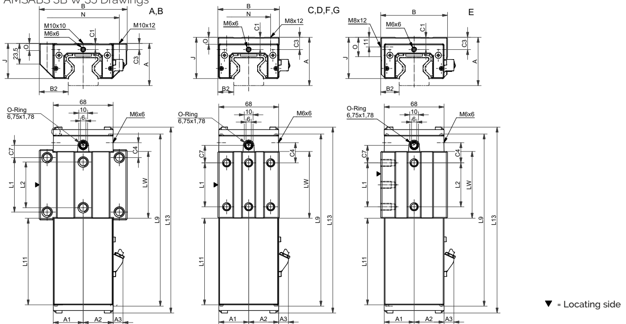
AMSABS 3B W B 35 Drawings
