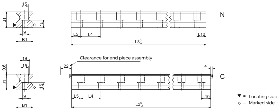
AMSABS 3B S 35 Drawings
